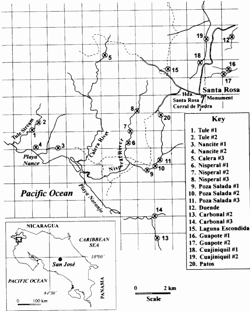
Fig. 1. Waterhole location in Guanacaste Conservation Area, Costa Rica.
